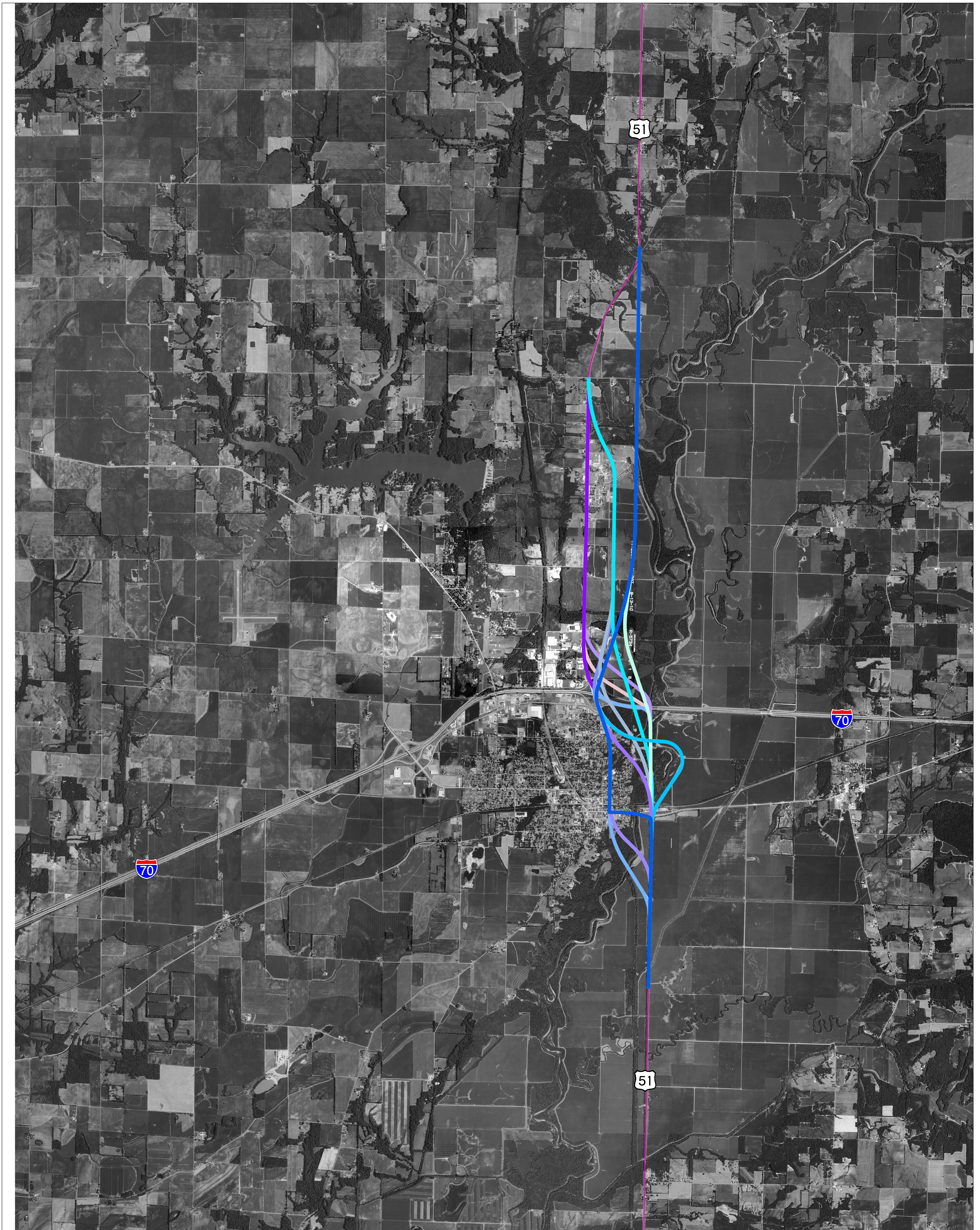
US 51 EIS Vandalia Alternatives - Eastern Brainstormed by CAG on August 31, 2010
